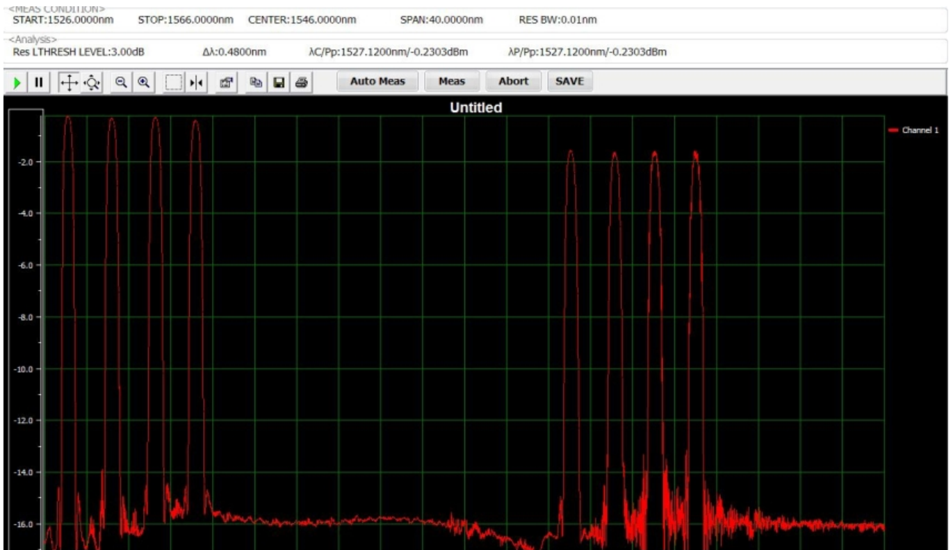
A Real Fiber Grating Sensor Sweep Spectrum
