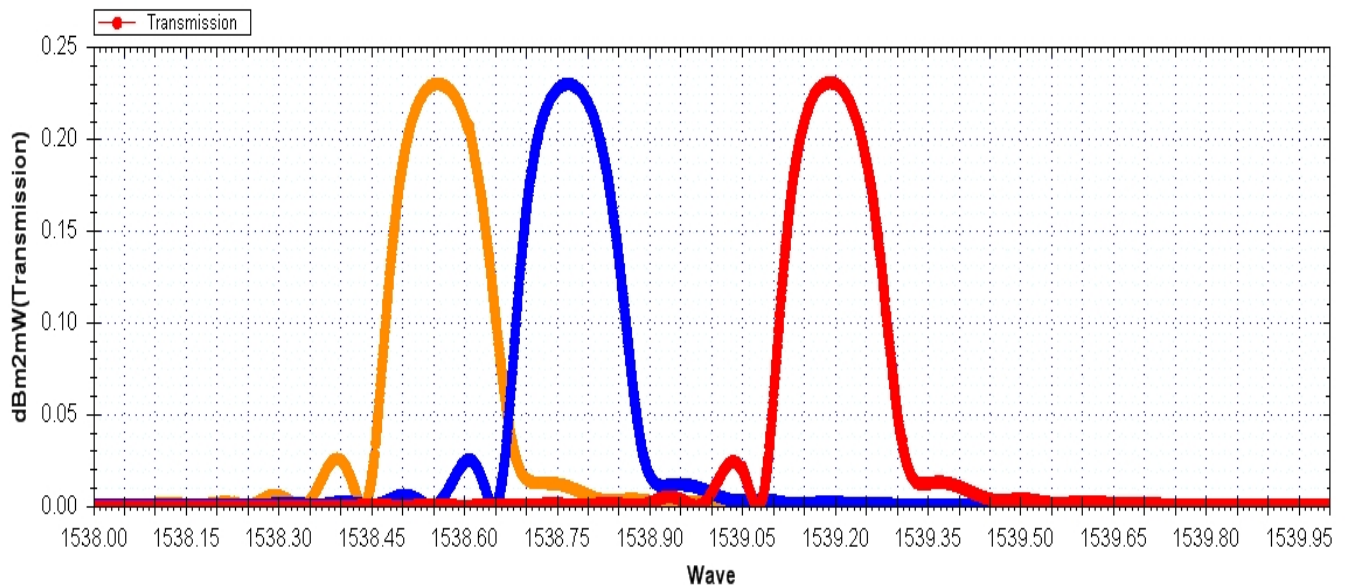
A Real Fiber Grating Sensor 0°, 23°, 100 °C Sweep Spectrum
